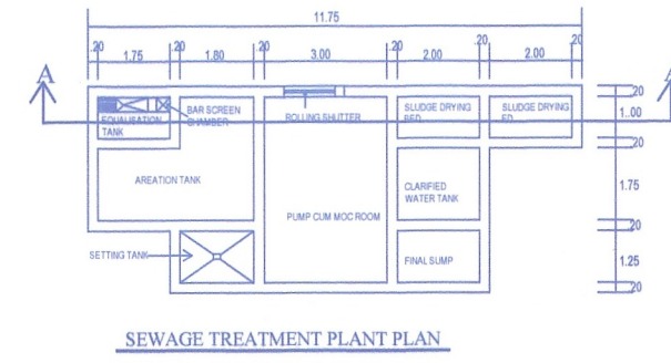
SEWAGE TREATMENT PLANT PLAN
