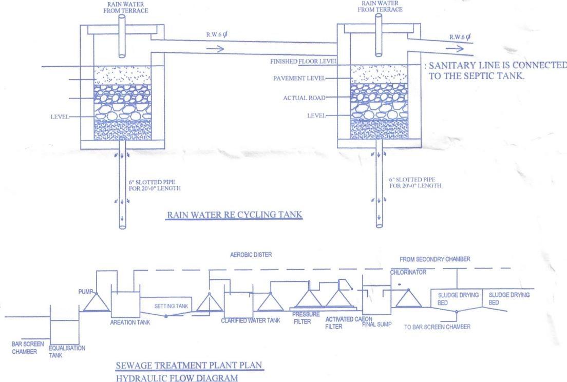
RAIN WATER RECYCLING TANK
