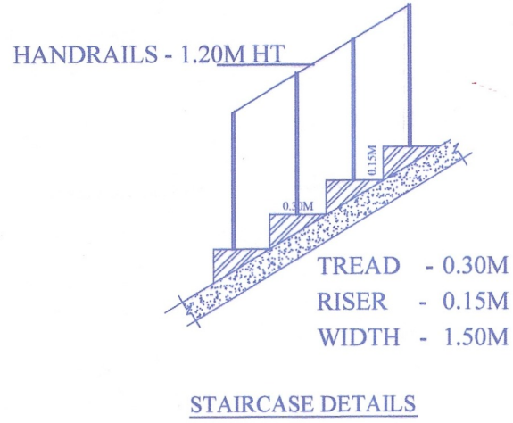
STAIRCASE DETAILS
