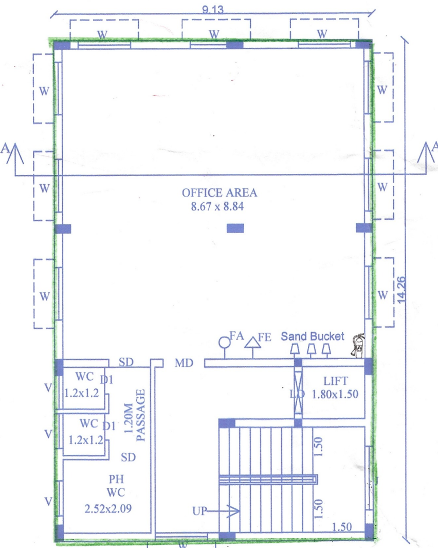
TYPICAL FLOOR PLAN (FIRST, SECOND AND THIRD FLOOR PLAN)
