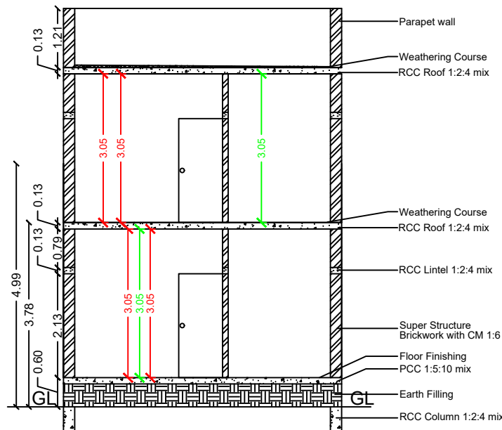
SECTION ON "VR"
