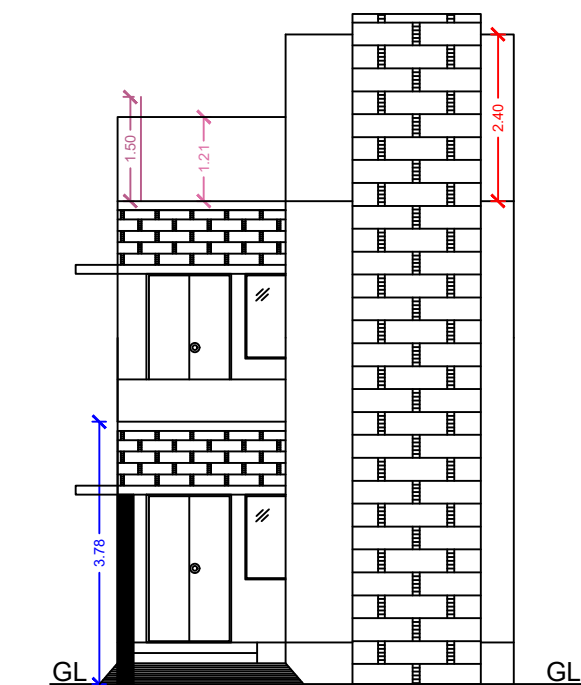
FRONT ELEVATION
