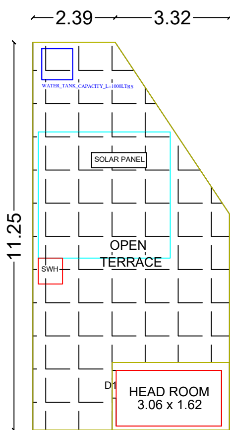
HEAD ROOM & TERRACE FLOOR PLAN
