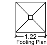
Footing Plan
