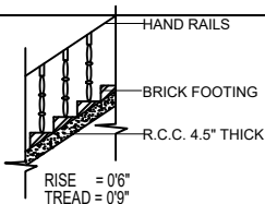
SECTION
