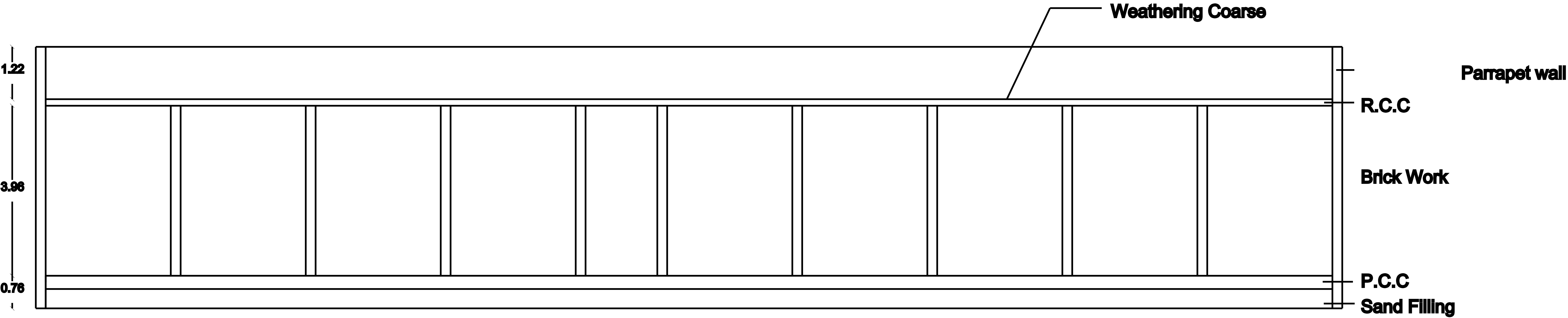
SECTION-A'-A'
