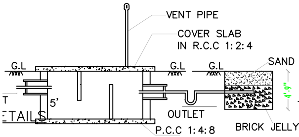
SECTION-AB
