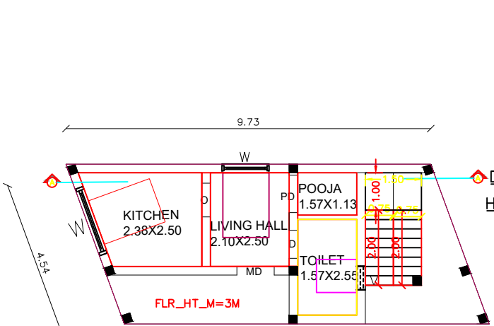
GROUND FLOOR
