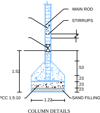
COLUMN DETAILS
