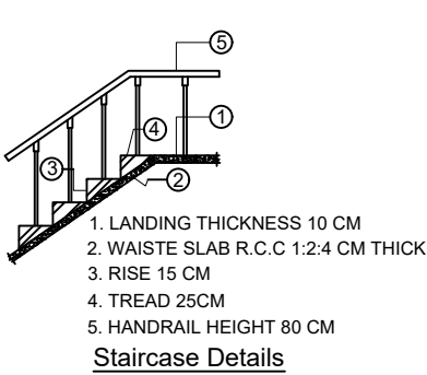
Staircase Details
