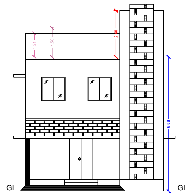
FRONT ELEVATION
