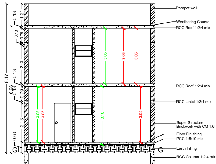
SECTION ON "VR"
