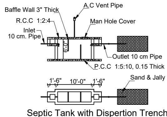
Septic Tank with Dispersion Trench
