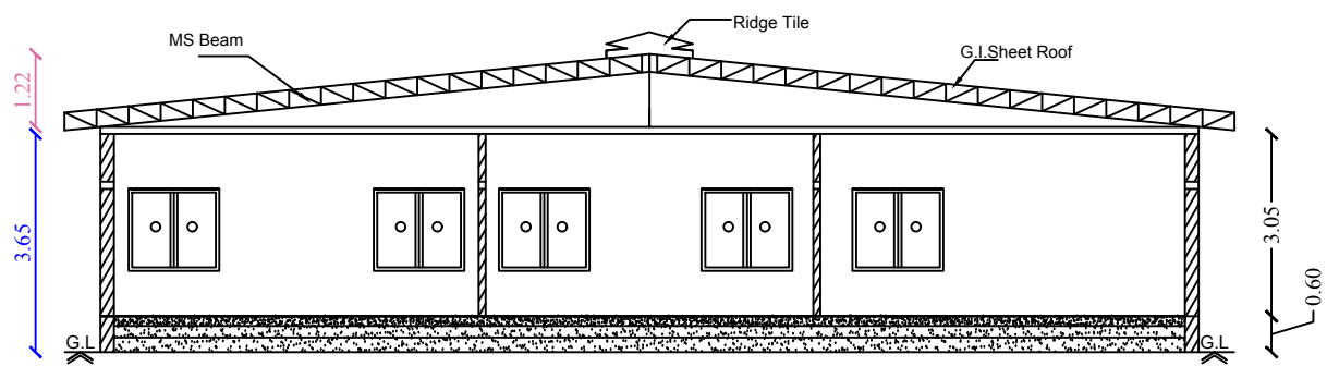
Section on-"AA"
