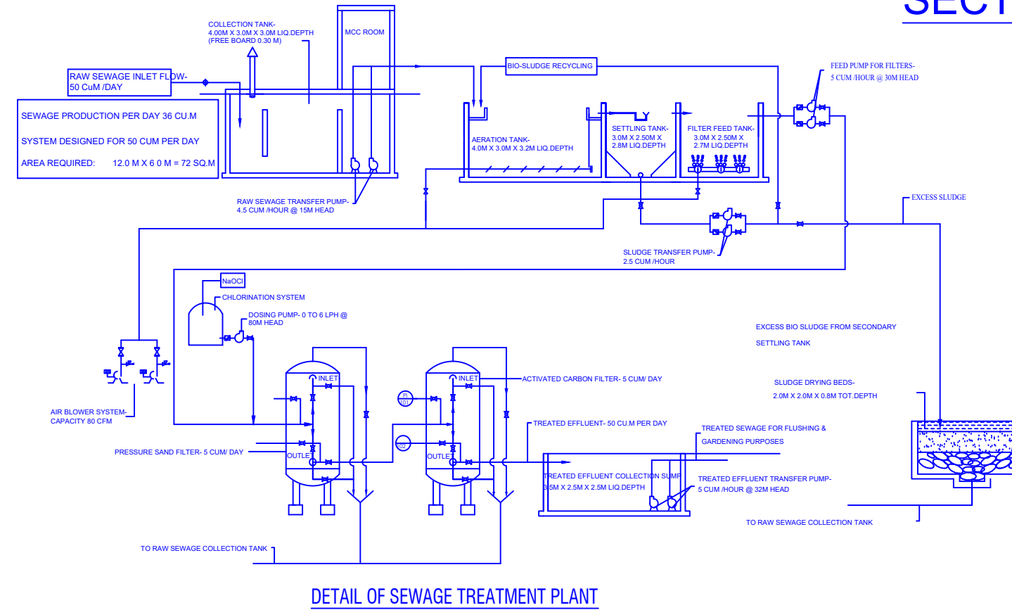
DETAIL OF SEWAGE TREATMENT PLANT
