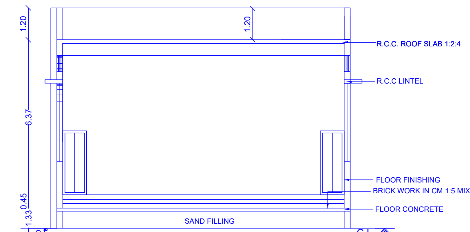
SECTION B-B
