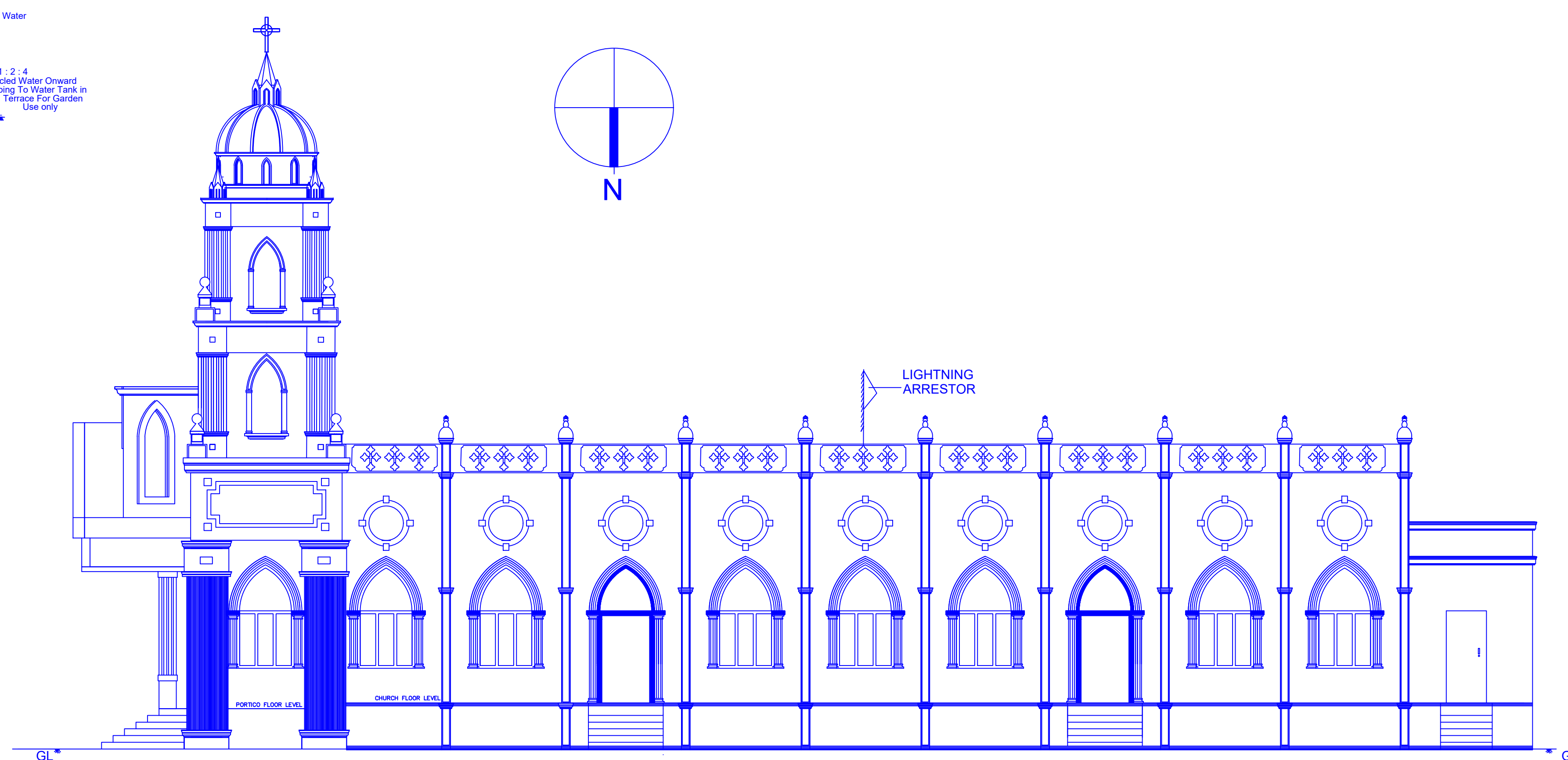
SIDE ELEVATION
