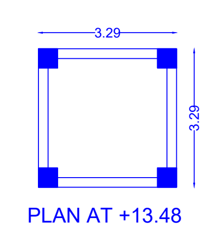
PLAN AT +13.48
