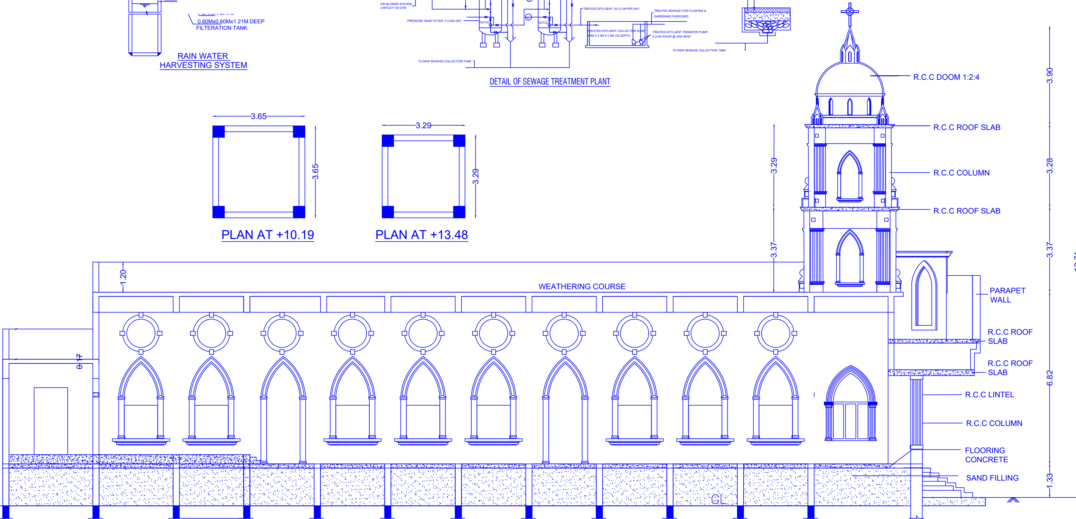
SECTION C-C
