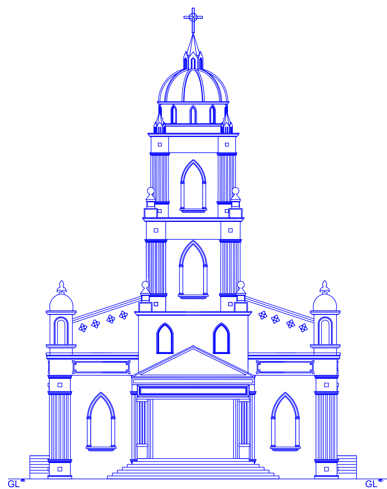
FRONT ELEVATION
