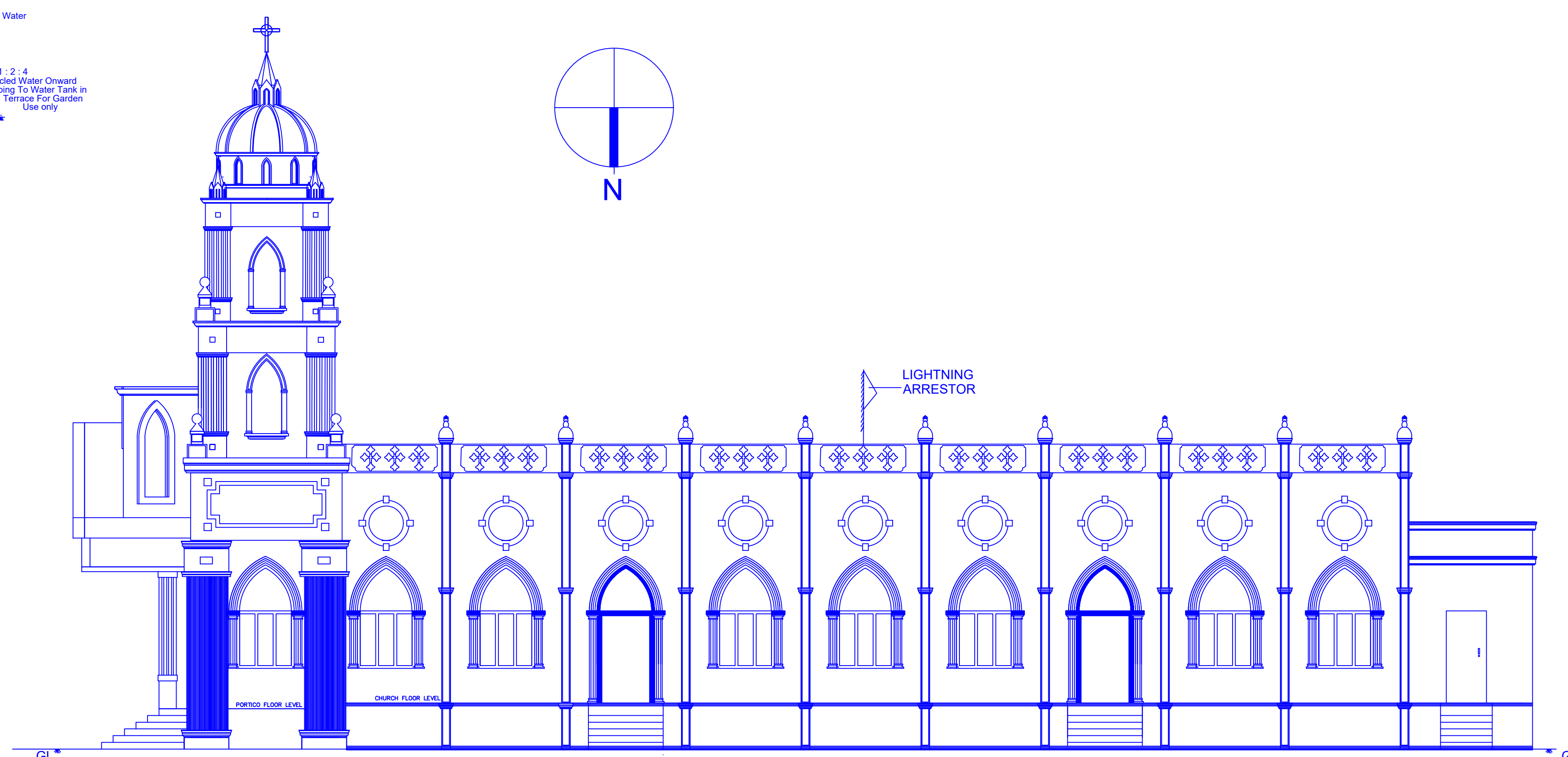
SIDE ELEVATION
