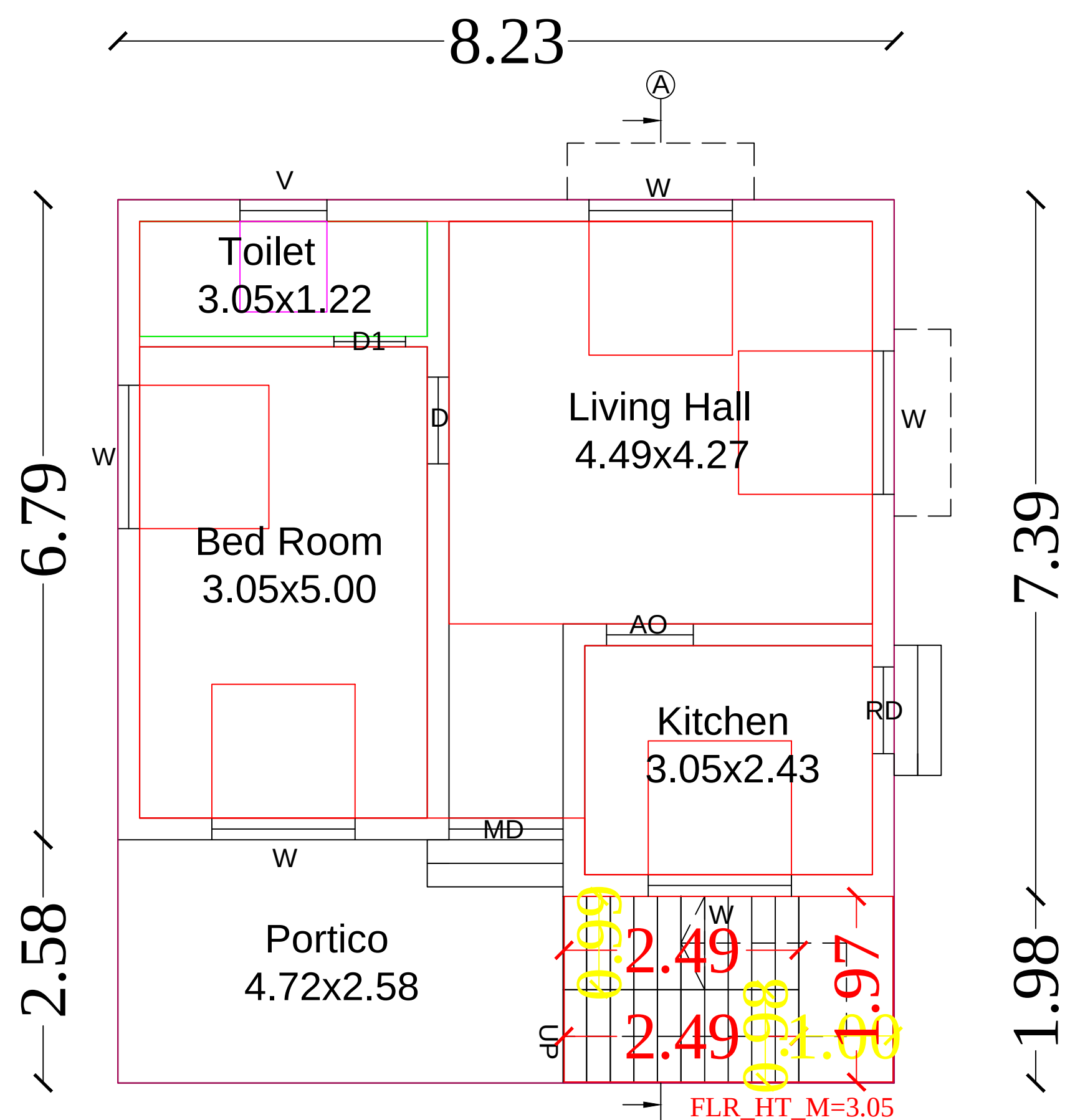
Ground Floor
