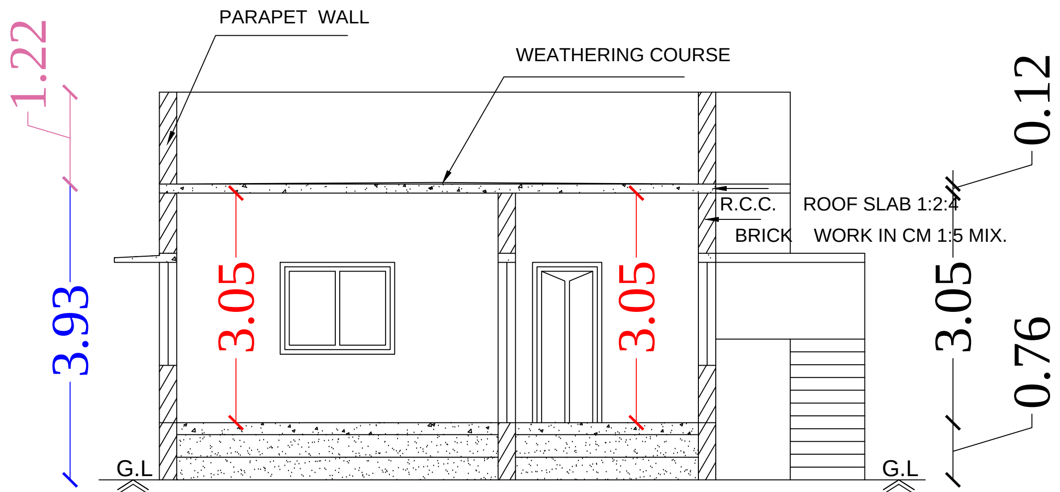
Section on-"AA"
