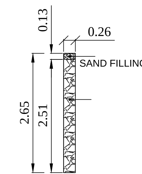
DETAILS OF PERCULATION PIT
