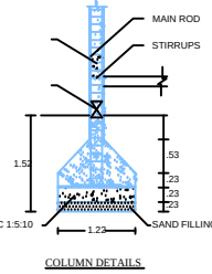
COLUMN DETAILS
