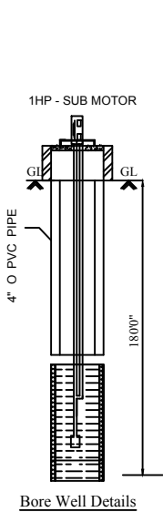
Bore Well Details
