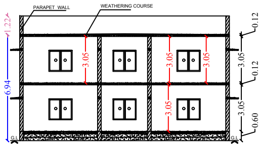
Section on-AA
