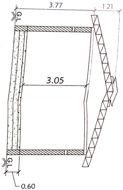
Section on-"AA"
