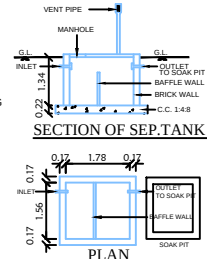
PLAN SEPTIC TANK
