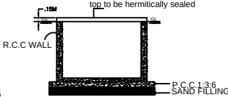
SECTION ON BB SCALE 1:100
