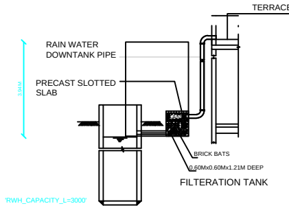
RAIN WATER HARVESTING SYSTEM SCALE 1:100
