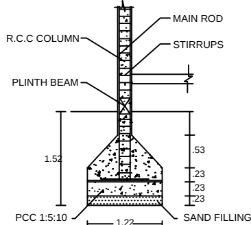
COLUMN DETAILS SCALE 1:100
