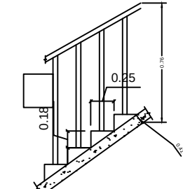
SECTION OF STAIRCASE SCALE 1:100
