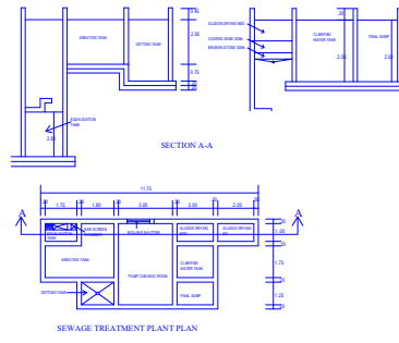
SEWAGE TREATMENT PLANT
