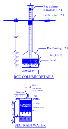
SEC. RAIN WATER HARVEST PIT
