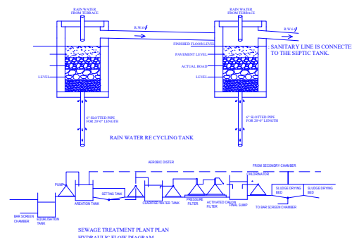
SEWAGE TREATMENT PLANT PLAN HYDRAULIC FLOW DIAGRAM
