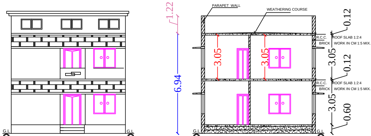
Front Elevation
