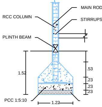
COLUMN DETAILS
