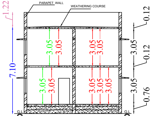
Section on-"AA"
