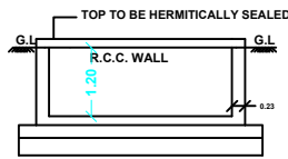
RWHS SECTION (SAMPLE) RWHS_CAPACITY_L = 2000
