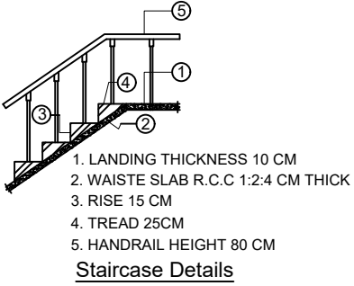
Staircase Details
