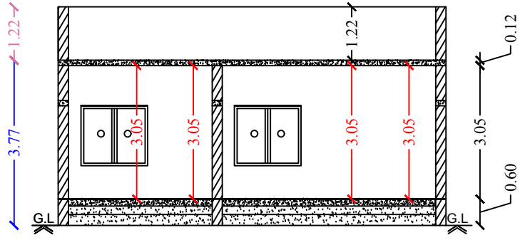
Section on-"AA"
