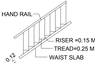
STAIRCASE DETAILS
