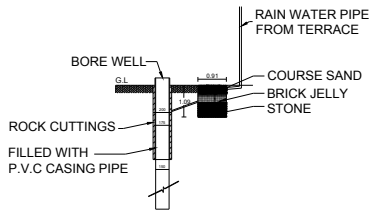
RAIN WATER HARVESTING DETAIL
