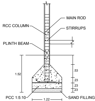
COLUMN DETAILS
