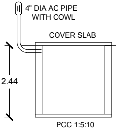
SEPTIC TANK
