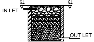
RAINWATER STORAGE PIT DETAILS
