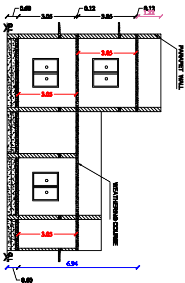
Section on-AA'
