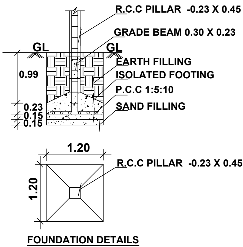
FOUNDATION DETAILS
