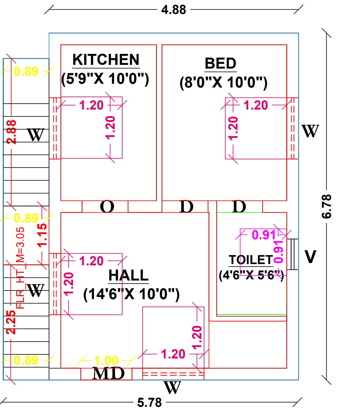
FLOOR-GROUND
