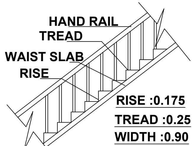
STAIRCASE DETAILS
