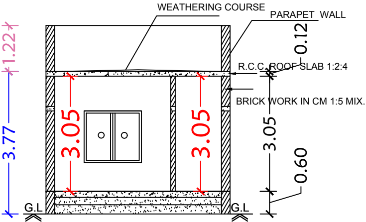
Section on-"AA"
