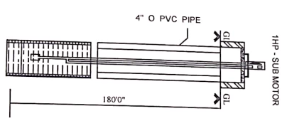
Bore Well Details
