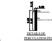
DETAILS OF PERCOLATION PIT
