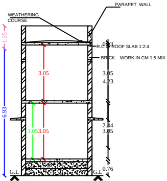
Section on-AA'
