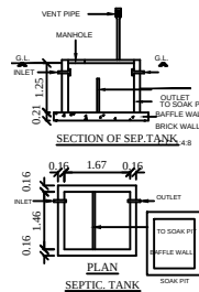
PLAN SEPTIC TANK
