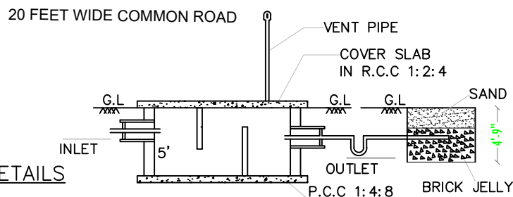
SECTION-AB
