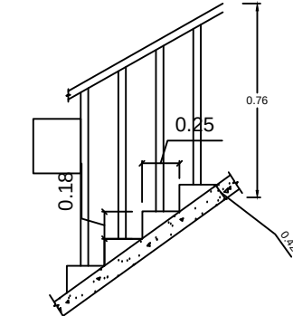
SECTION OF STAIRCASE SCALE 1:100
