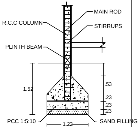
COLUMN DETAILS SCALE 1:100
