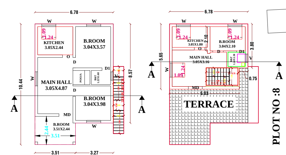
EXI.GROUND FLOOR PLAN
