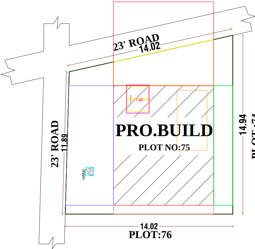
SITE PLAN
