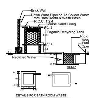
DETAILS FOR BATH ROOM WASTE WATER FILTRATION SYSTEM & SEPTIC TANK
