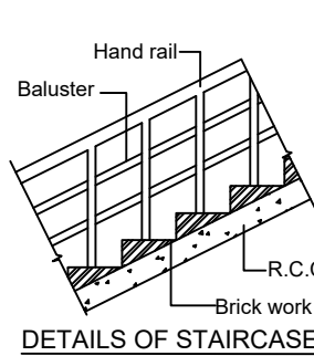
DETAILS OF STAIRCASE
