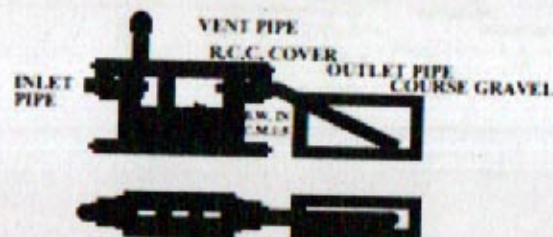
SEPTIC TANK & OF DISPERSION TRENCH DETAILS
