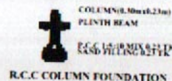
R.C.C COLUMN FOUNDATION
