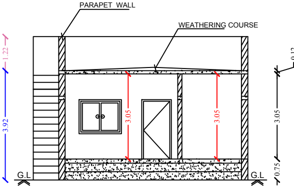
Section on-"AA"
