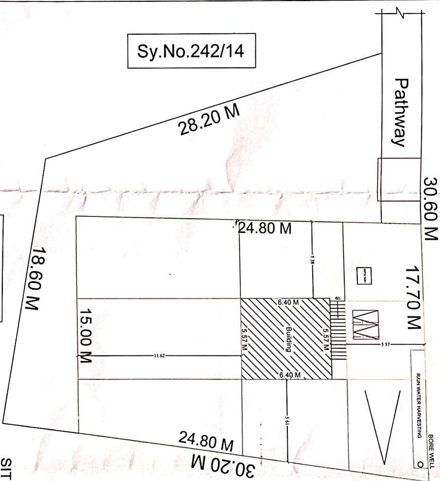
RAIN WATER HARVESTING SYSTEM
