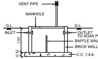
SECTION OF SEP.TANK
