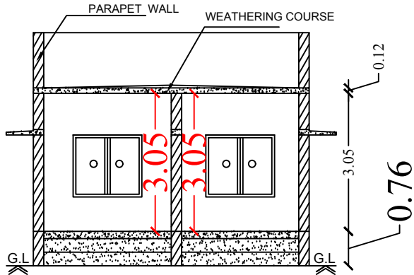
Section on-"AA"
