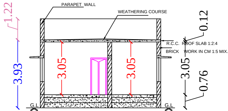
Section on-"AA"
