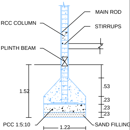
COLUMN DETAILS
