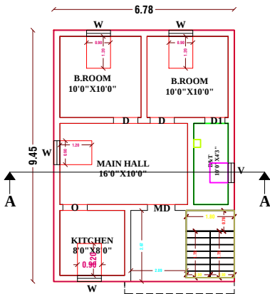
PRO.GROUND FLOOR PLAN
