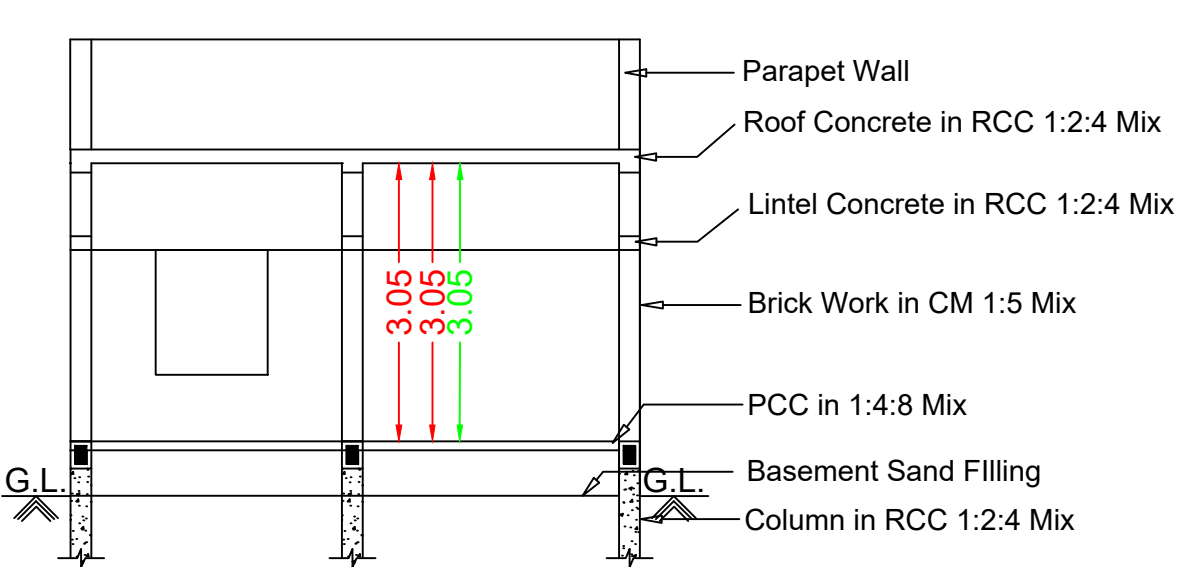
Section RR
