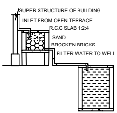
RAINWATER HARVESTING SYSTEM RWH_CAPACITY_L = 2000
