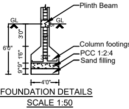
FOUNDATION DETAILS SCALE 1:50
