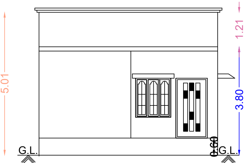
Front Elevation
