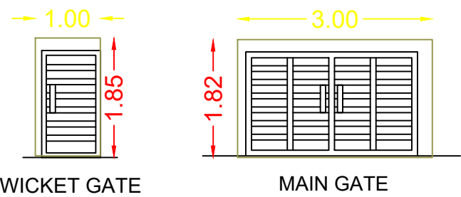
WICKET GATE
