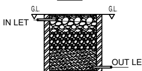
RAINWATER STORAGE PIT DETAILS
