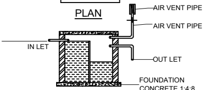
SEPTIC TANK DETAILS
