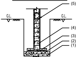
FOOTING DETAILS
