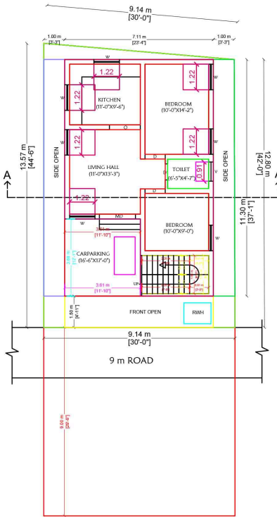
PRO. GROUND FLOOR PLAN
