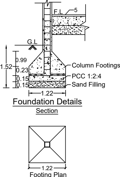
Footings Plan
