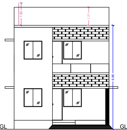
FRONT ELEVATION
