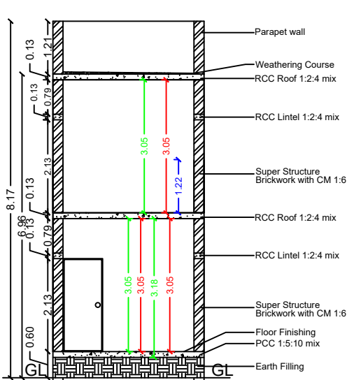
SECTION ON "VR"
