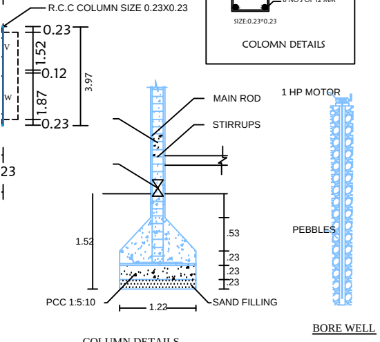
COLUMN DETAILS
