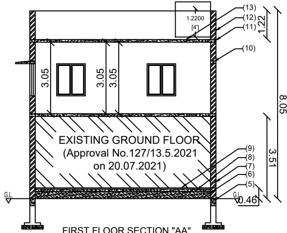
FIRST FLOOR SECTION "AA"
