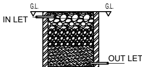
RAINWATER STORAGE PIT DETAILS
