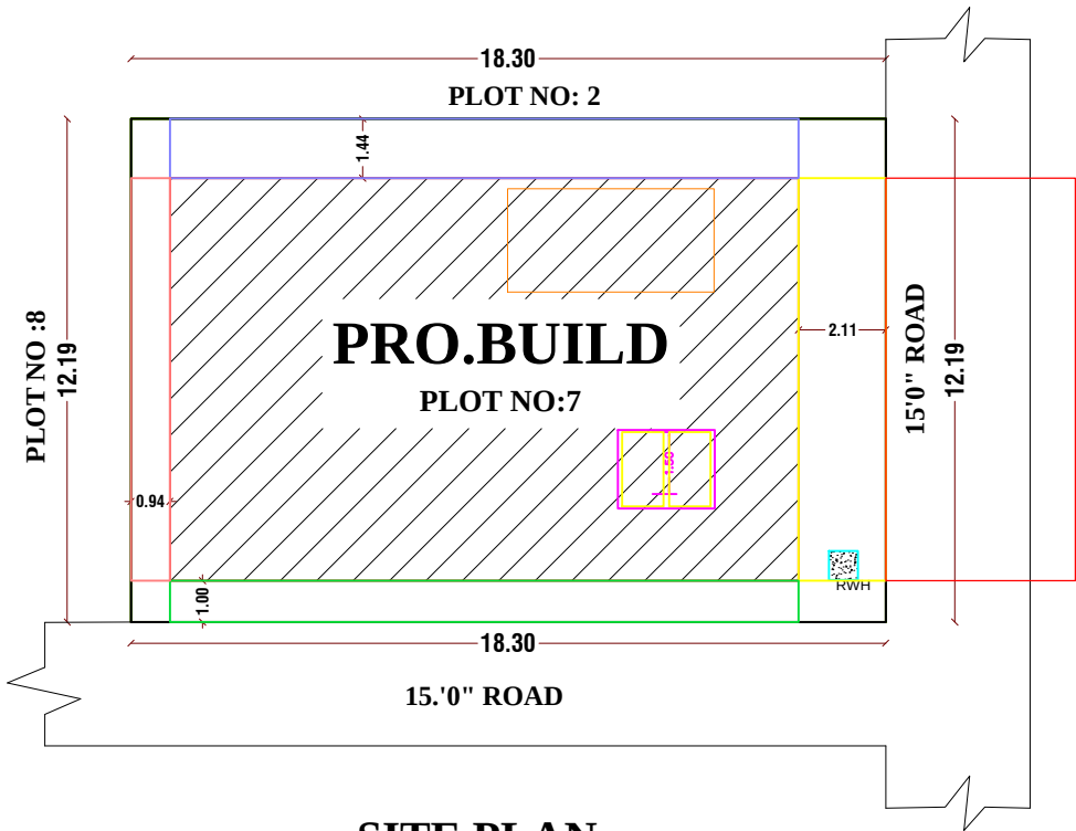
SITE PLAN
