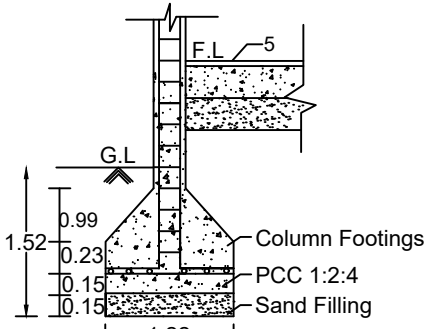
Foundation Details Section
