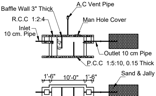
Septic Tank with Dispersion Trench
