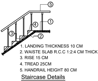
Staircase Details
